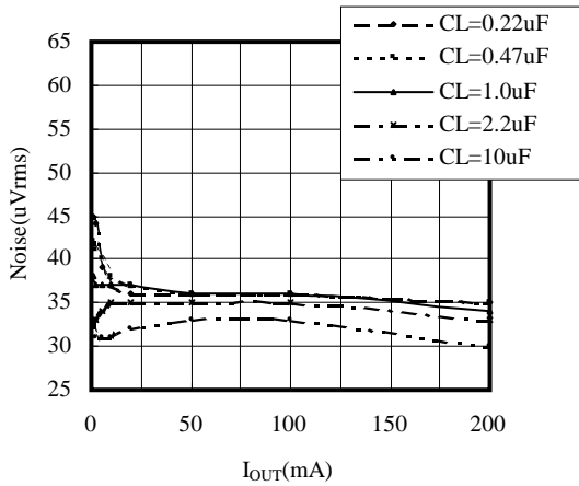
■ Output Noise vs. Output Current C_L=Tantal, C_{NP}=0.01\mu F
