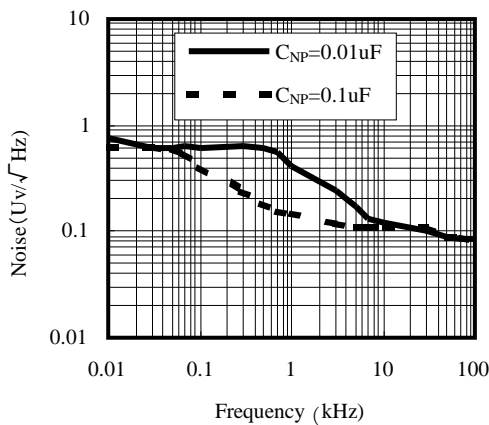
■ Output Noise Level(1/f) vs. Frequency I_{OUT}=10mA, C_{IN}=10\mu F, C_L=0.22\mu F (MLCC)
