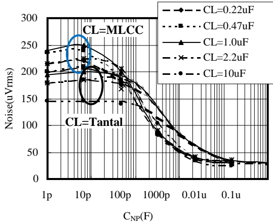
■ Output Noise vs. Noise Pass Capacitance I_{OUT}=30mA
