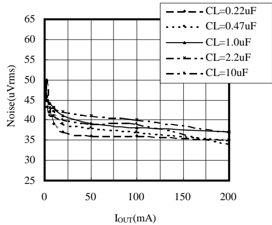
■ Output Noise vs. Output Current C_L=MLCC, C_{NP}=0.01\mu F
