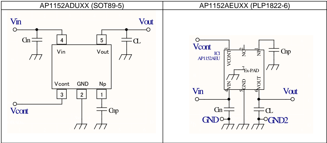
Figure 6. External connection circuit example
