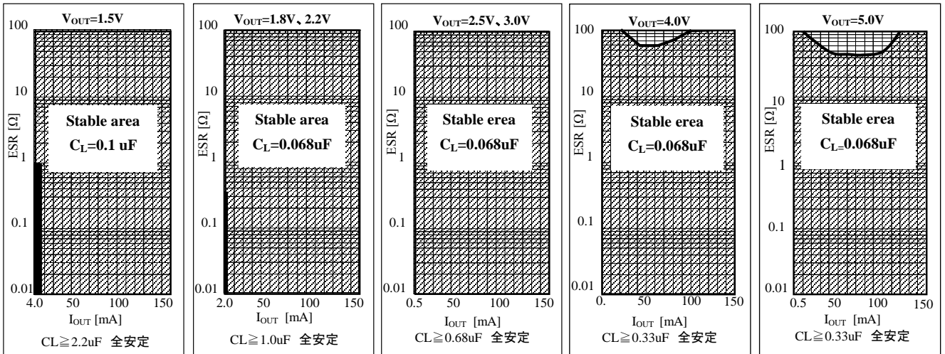
Figure 3. Stable operation area vs. voltage, current, and ESR
