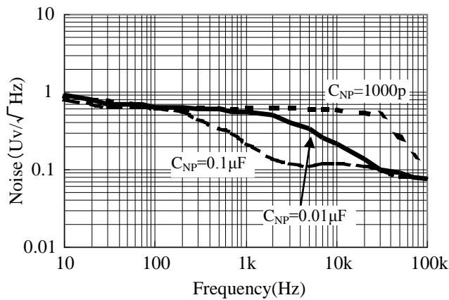
■ Output Noise Level(1/f) vs. Frequency I_{OUT}=10mA, C_{IN}=10\mu F, C_L=0.22\mu F(MLCC)
