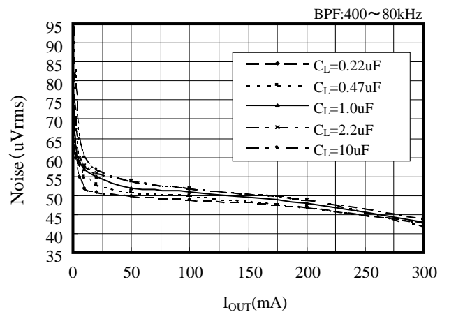
■ Noise vs. Output Current C_L=MLCC, C_{NP}=10000pF
