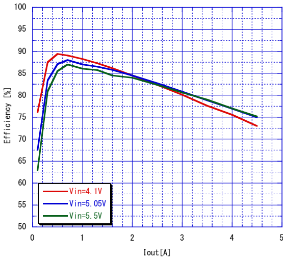
Figure 10. Efficiency
