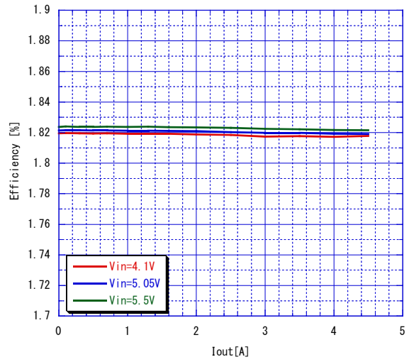
Figure 11. Load Regulation
