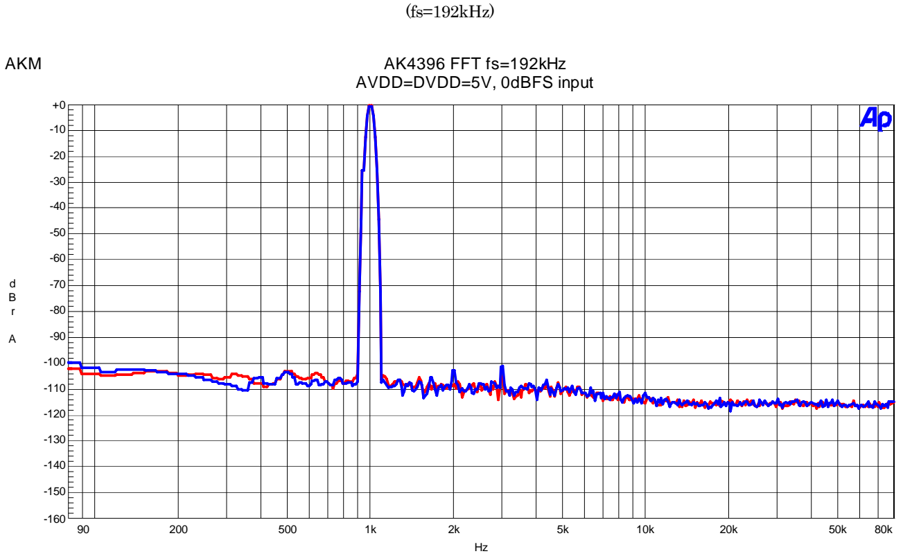
Figure 27 FFT (fin=1kHz, Input Level=0dBFS)
