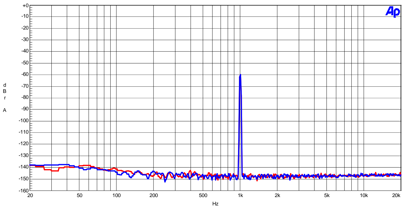
Figure 10 FFT (fin=1kHz, Input Level=-60dBFS)
