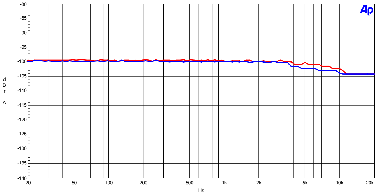
AK4396 THD+N vs Input Frequency fs=44.1kHz AVDD=DVDD=5V, 0dBFS input
