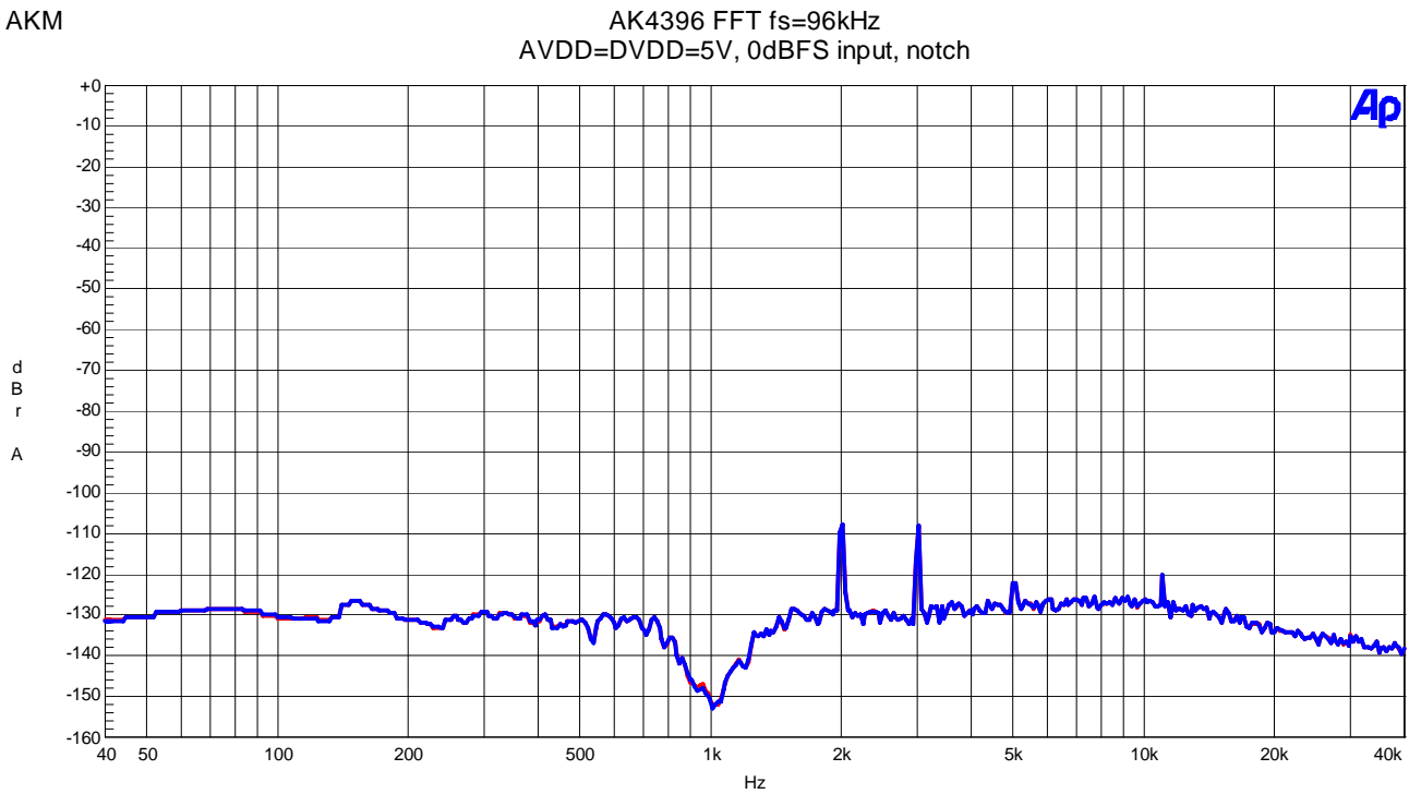
Figure 19 FFT(fin=1kHz, Input Level=0dBFS, Notch)
