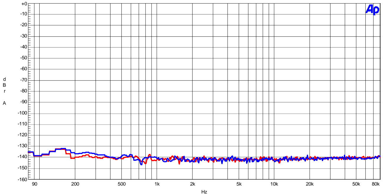
Figure 30 FFT (Noise Floor)
