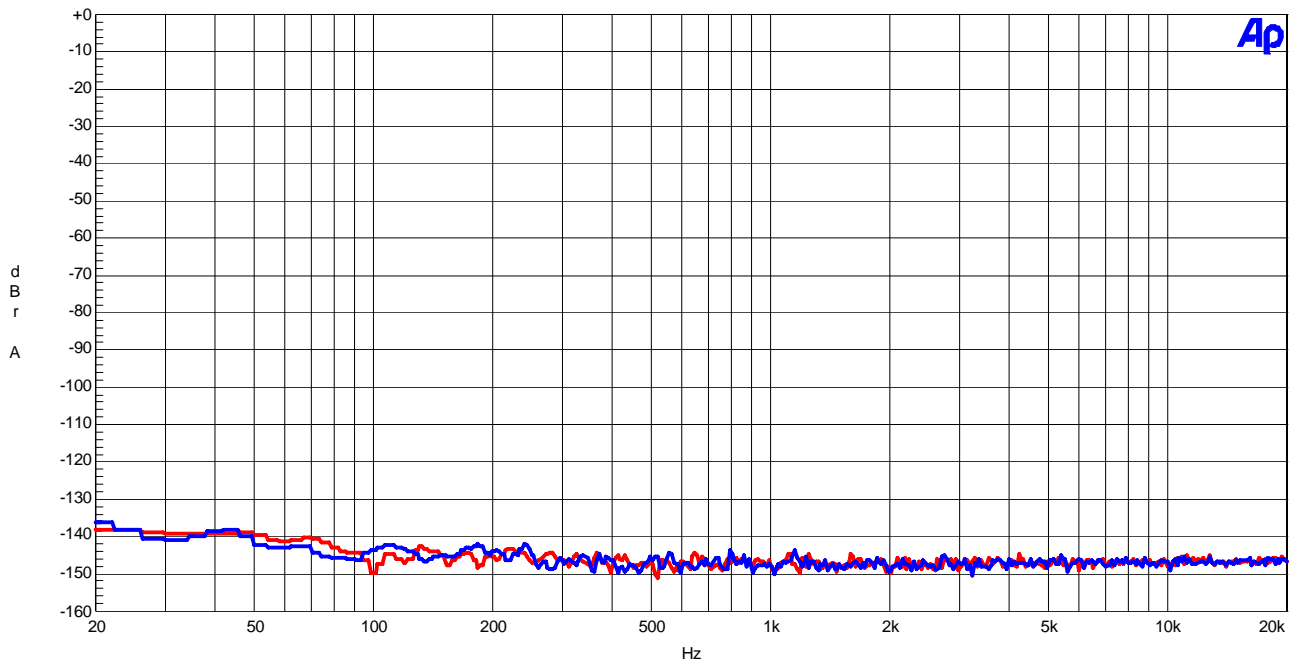
Figure 11 FFT (Noise Floor)
