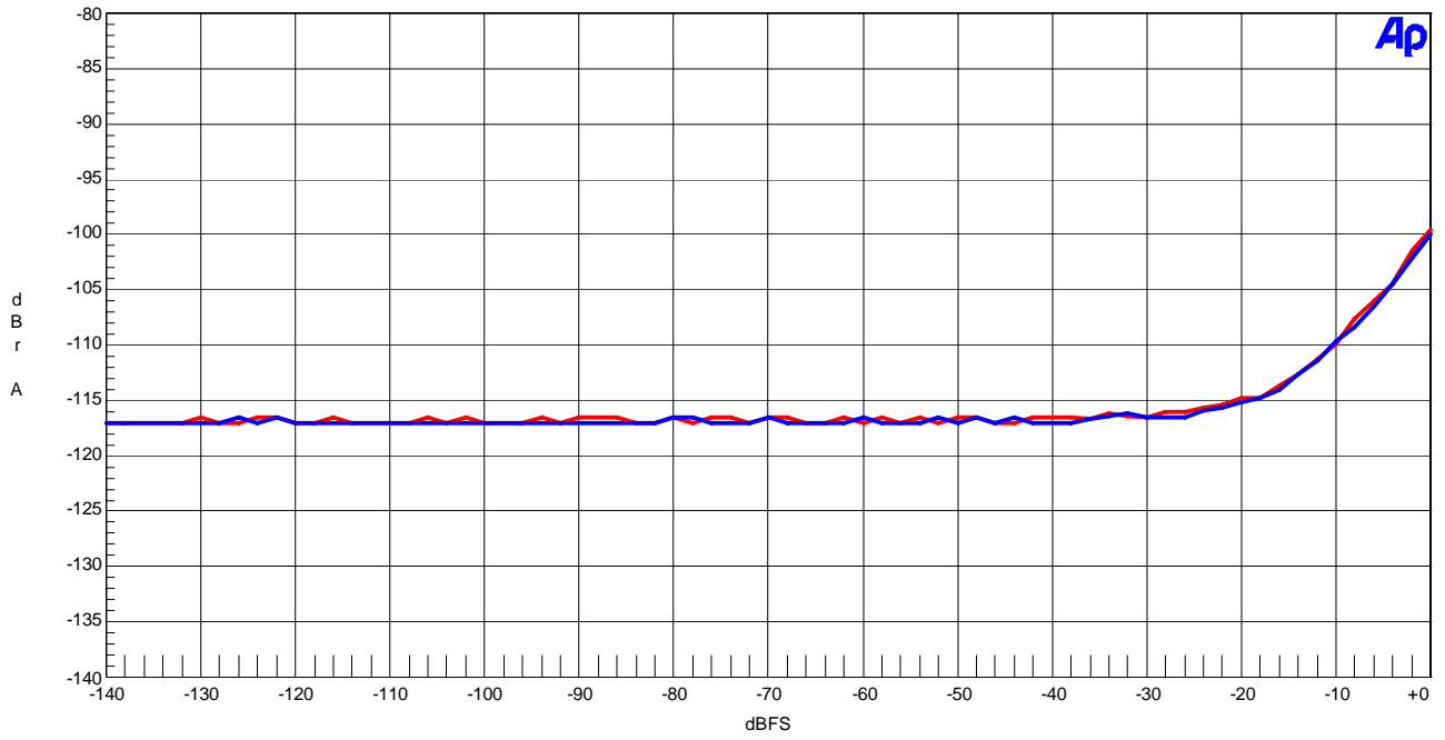
AK4396 THD+N vs Input Level fs=44.1kHz AVDD=DVDD=5V, 0dBFS
