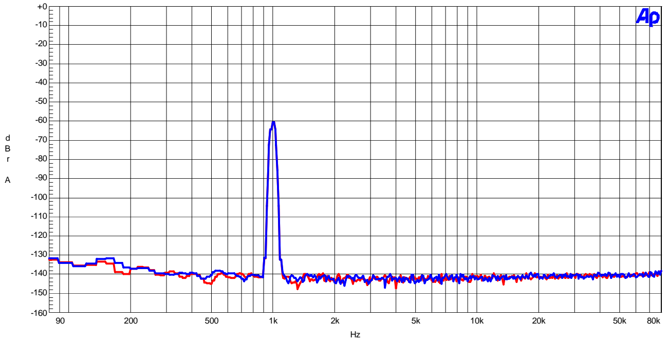
Figure 29 FFT (fin=1kHz, Input Level=-60dBFS)
