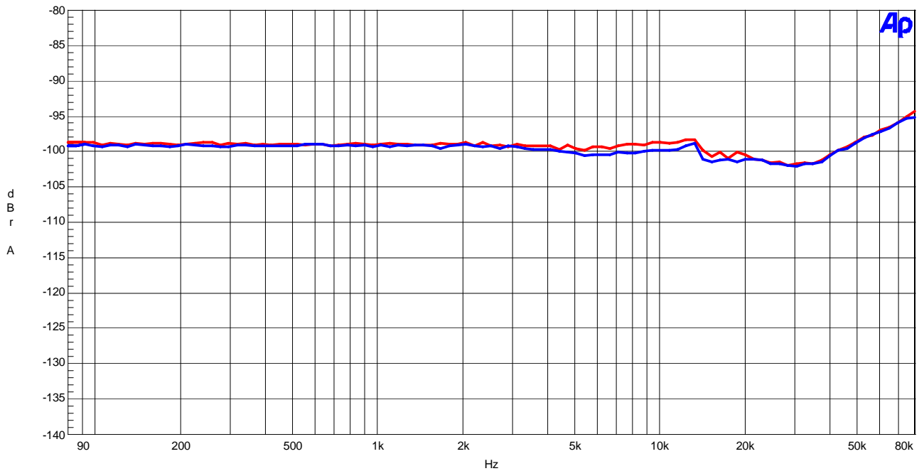
AK4396 THD+N vs Input Frequency fs=192kHz AVDD=DVDD=5V, 0dBFS input
