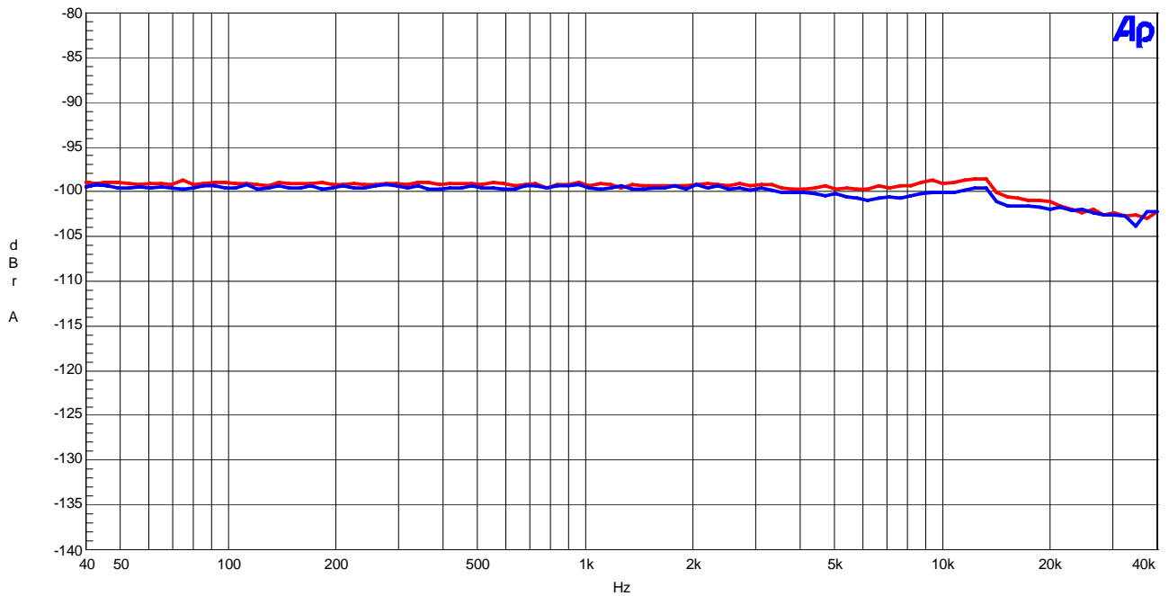
AK4396 THD+N vs Input Frequency fs=96kHz AVDD=DVDD=5V, 0dBFS input
