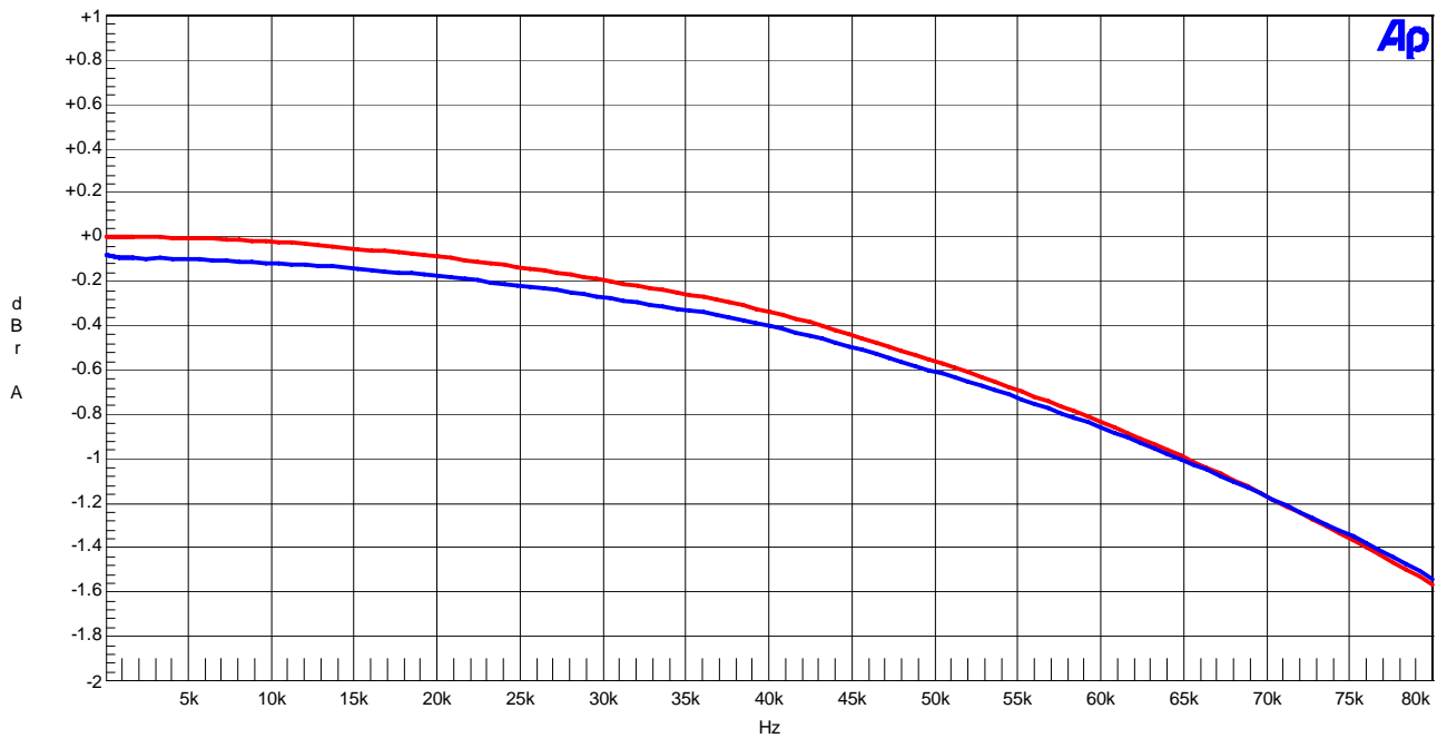
Figure 34 Frequency Response (Input level=0dBFS)
