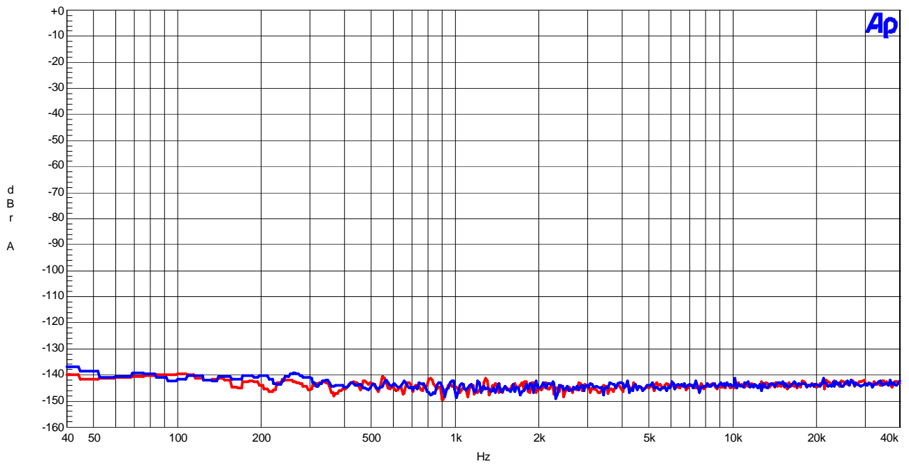
Figure 21 FFT (Noise Floor)
