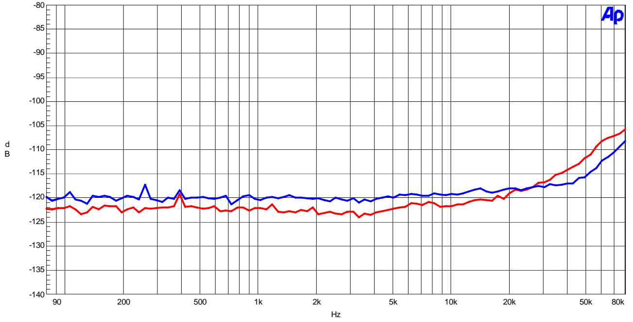
Figure 35 Crosstalk (Input level=0dBFS)
