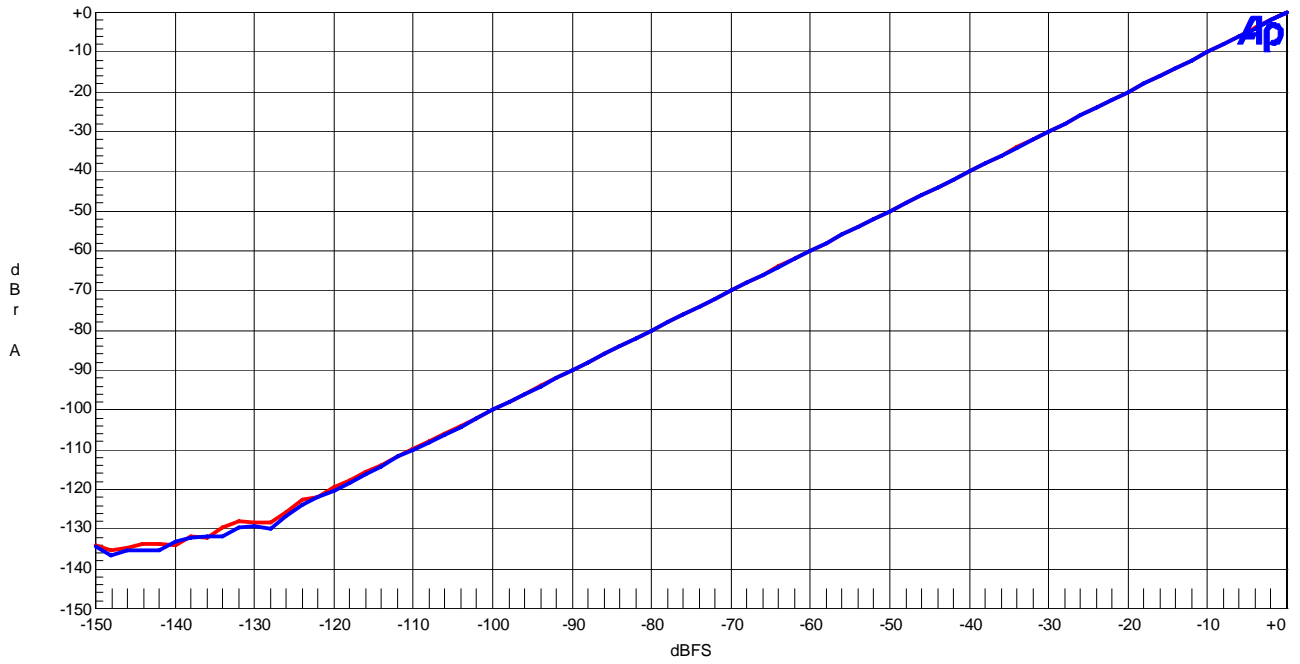
Figure 24 Linearity (fm=1kHz)
