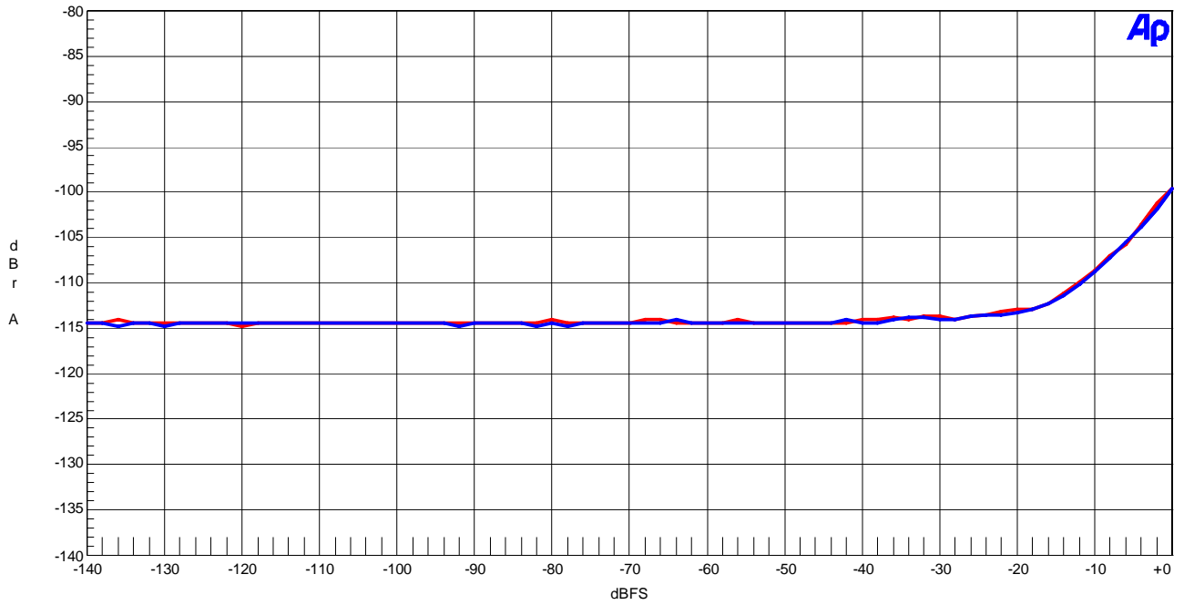
AK4396 THD+N vs Input Level fs=96kHz AVDD=DVDD=5V, 0dBFS input
