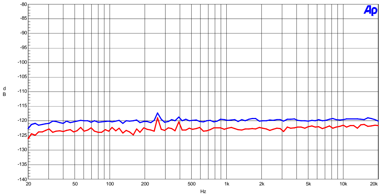
Figure 17 Crosstalk (Input level=0dBFS)
