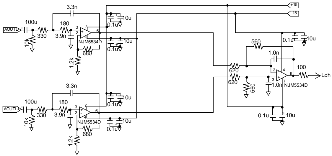
Figure 4 External Analog Filter
