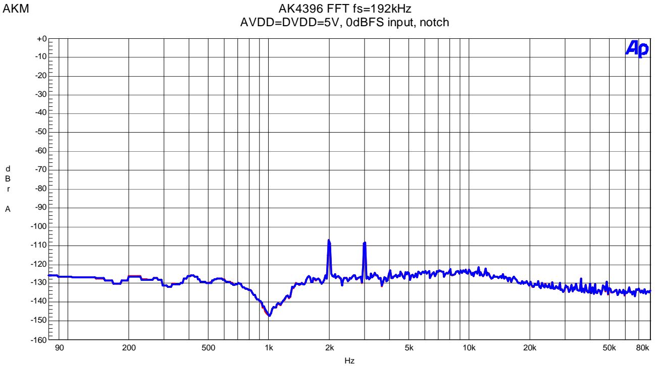
Figure 28 FFT(fin=1kHz, Input Level=0dBFS, Notch)
