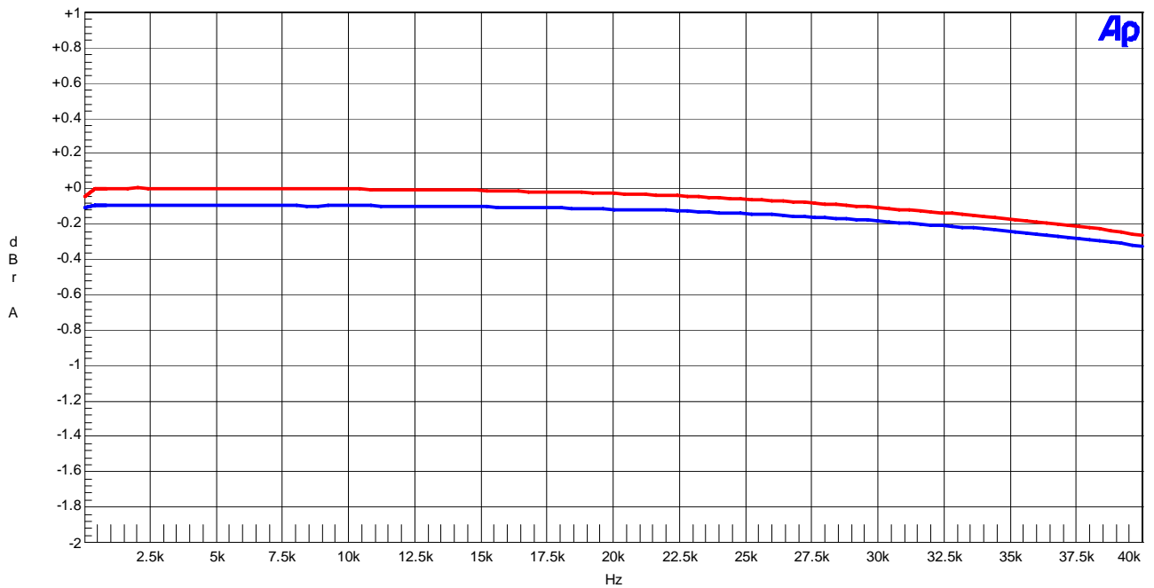
Figure 25 Frequency Response (Input level=0dBFS)
