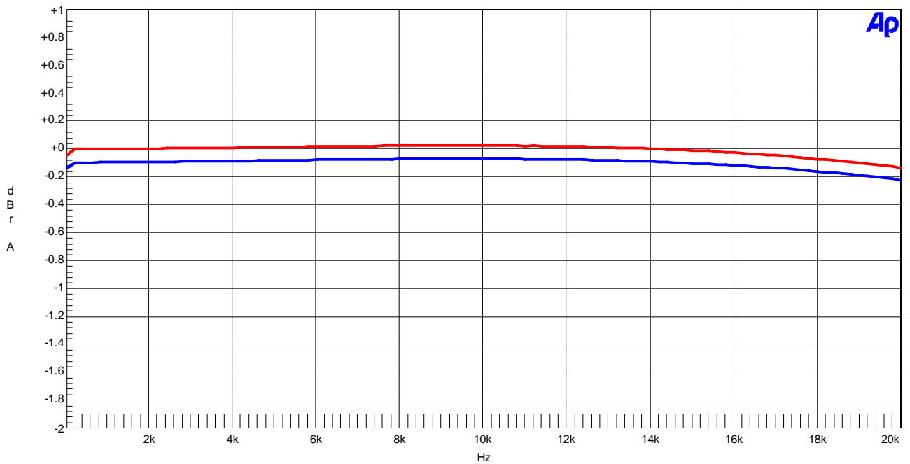
Figure 16 Frequency Response (Input level=0dBFS)
