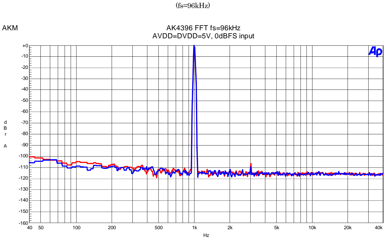
Figure 18 FFT (fin=1kHz, Input Level=0dBFS)
