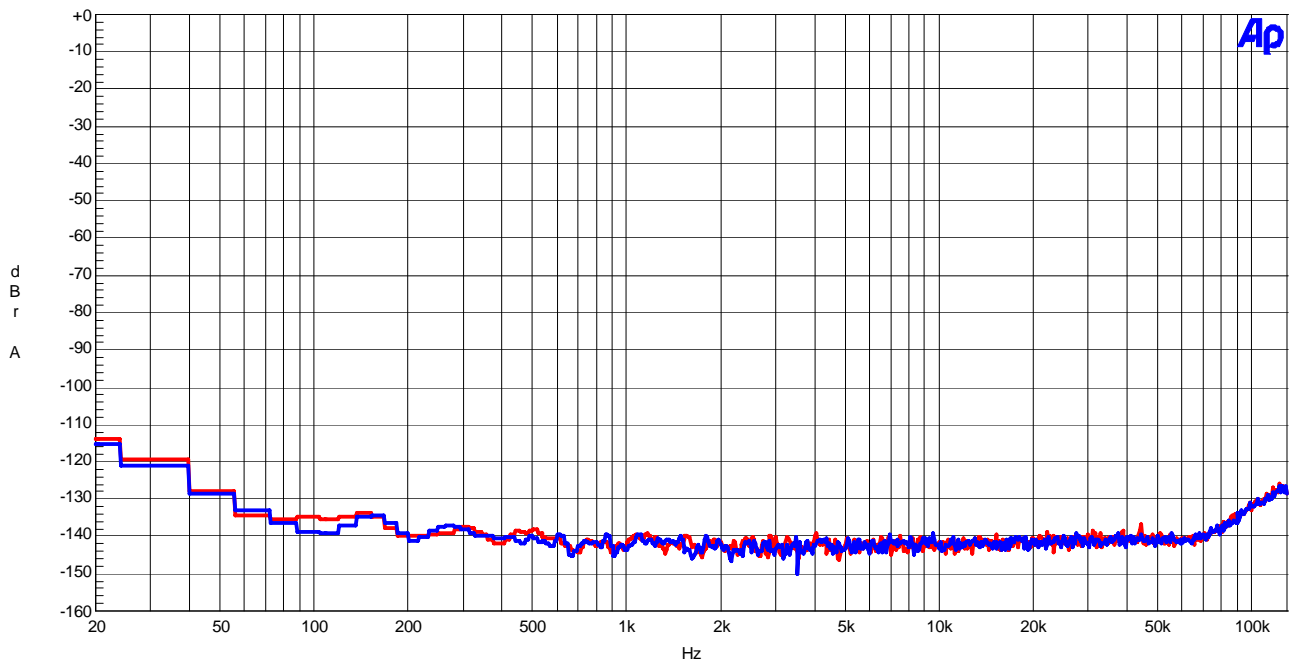
Figure 12 FFT (Out of band noise)
