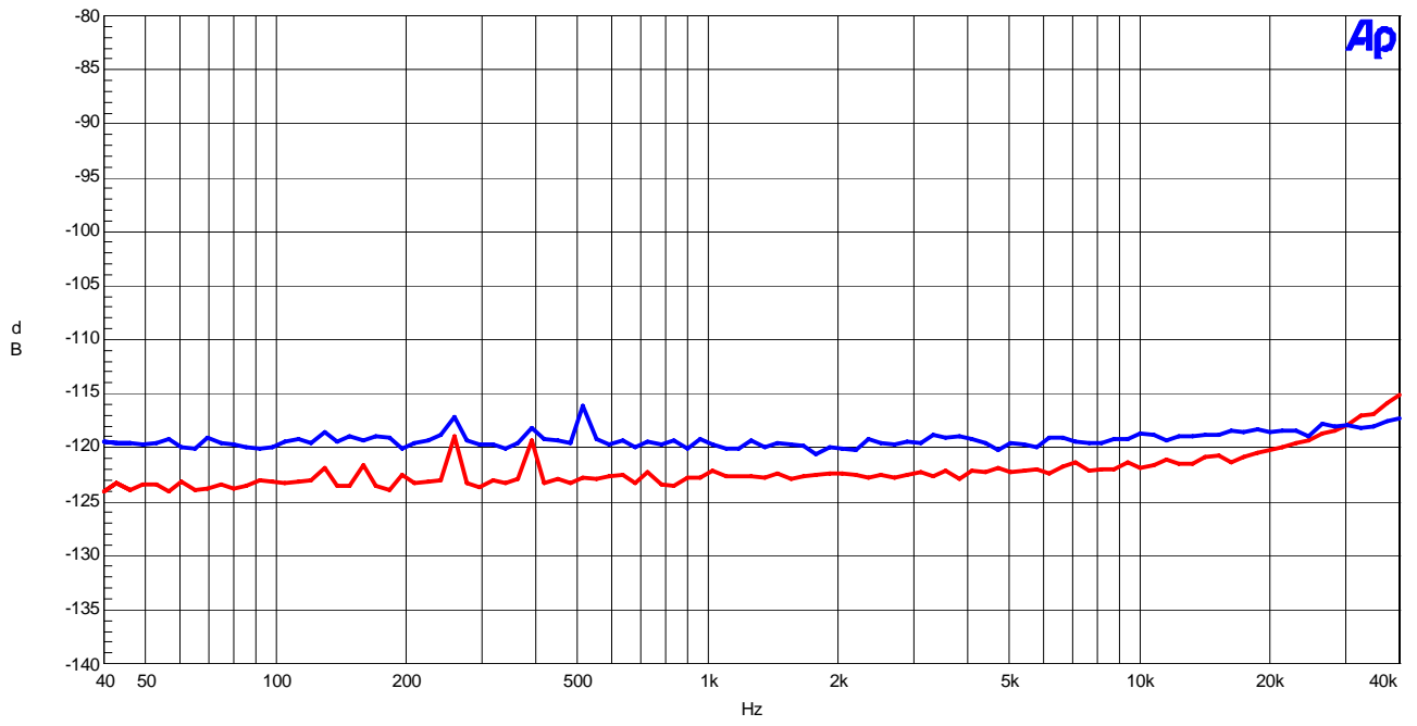
Figure 26 Crosstalk (Input level=0dBFS)
