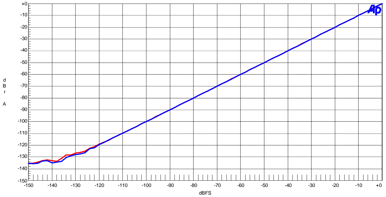
Figure 15 Linearity (fin=1kHz)
