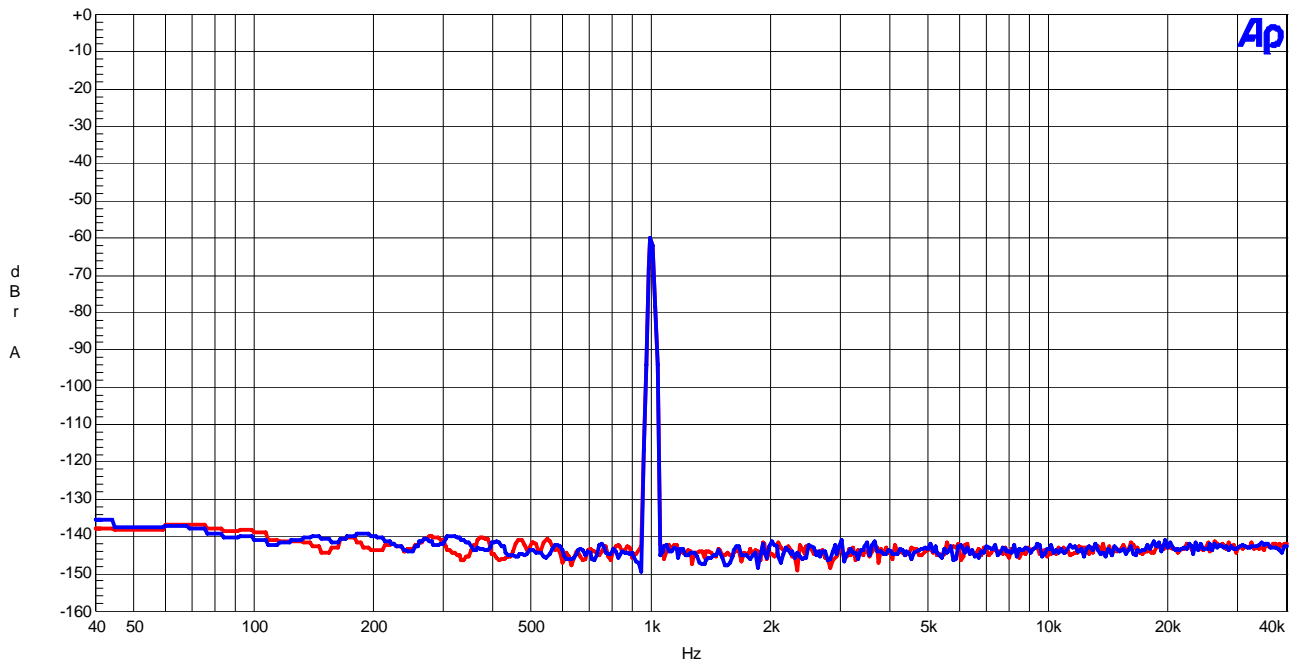
Figure 20 FFT (fin=1kHz, Input Level=-60dBFS)
