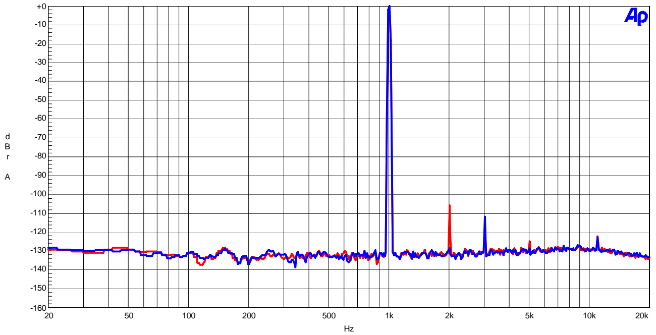
Figure 9 FFT (fin=1kHz, Input Level=0dBFS)
