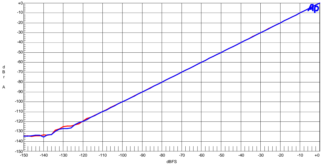
Figure 33 Linearity ( f_m=1\text{kHz} )
