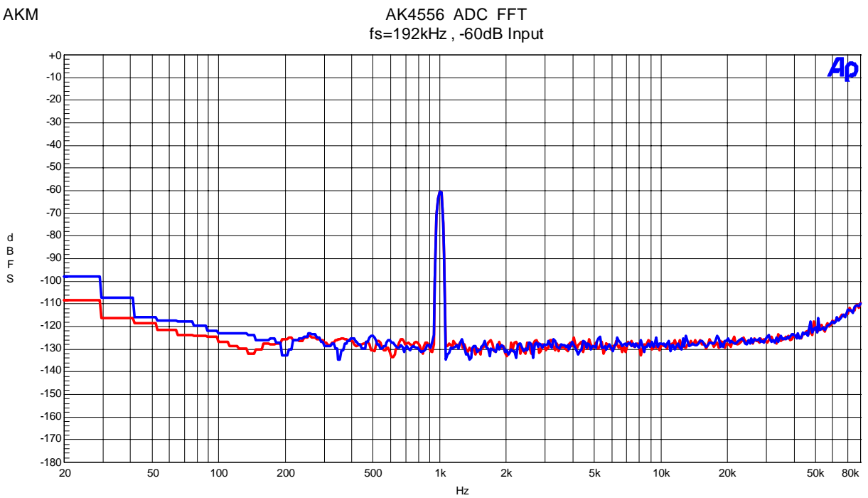
Figure 21. FFT (fin=1kHz , Input Level=-60dBFS)
