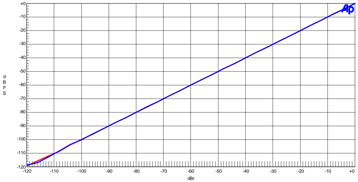
Figure 25. Linearity (fin=1kHz)
