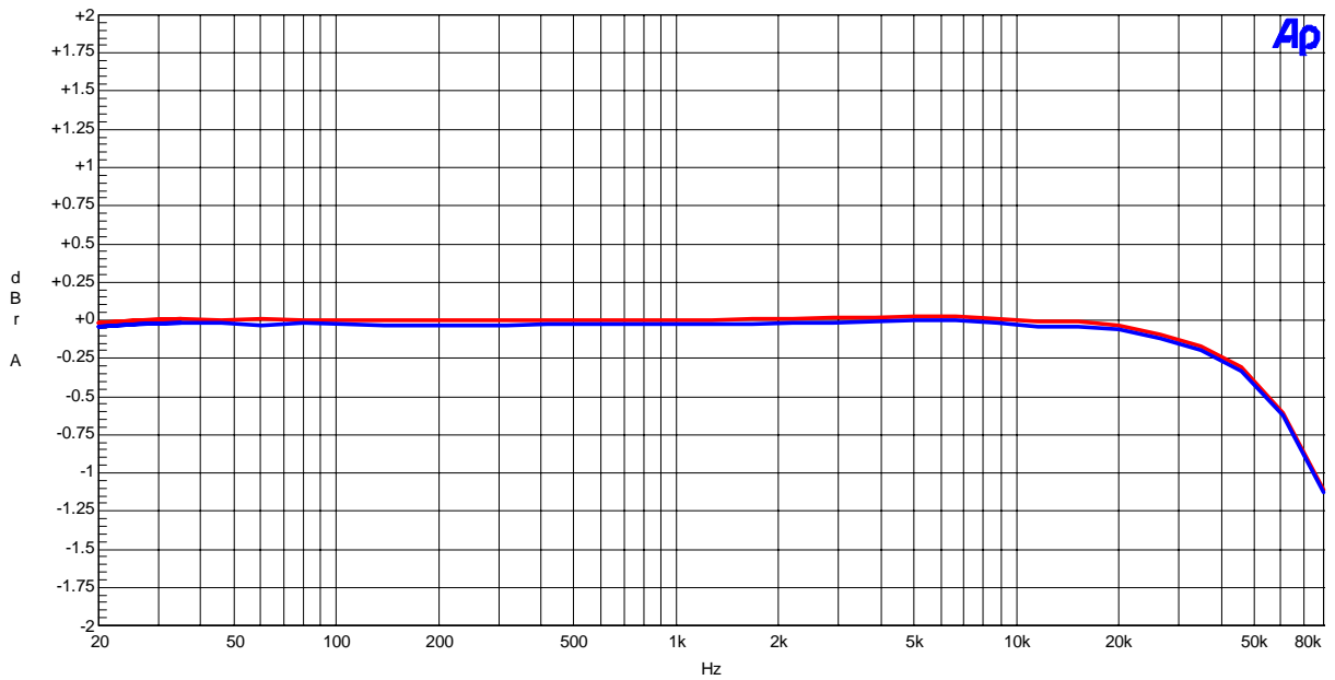
Figure 53. Frequency Response
