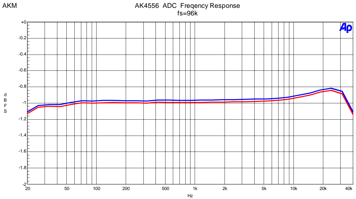
Figure 18. Frequency Response
