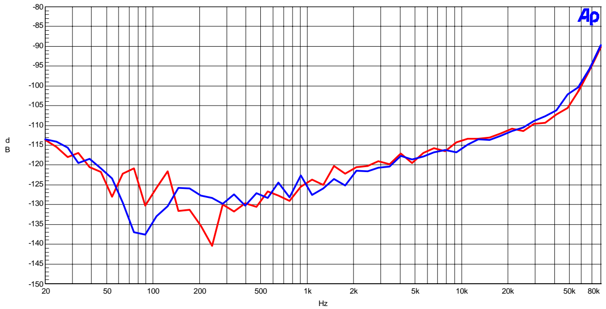
Figure 27. Crosstalk
