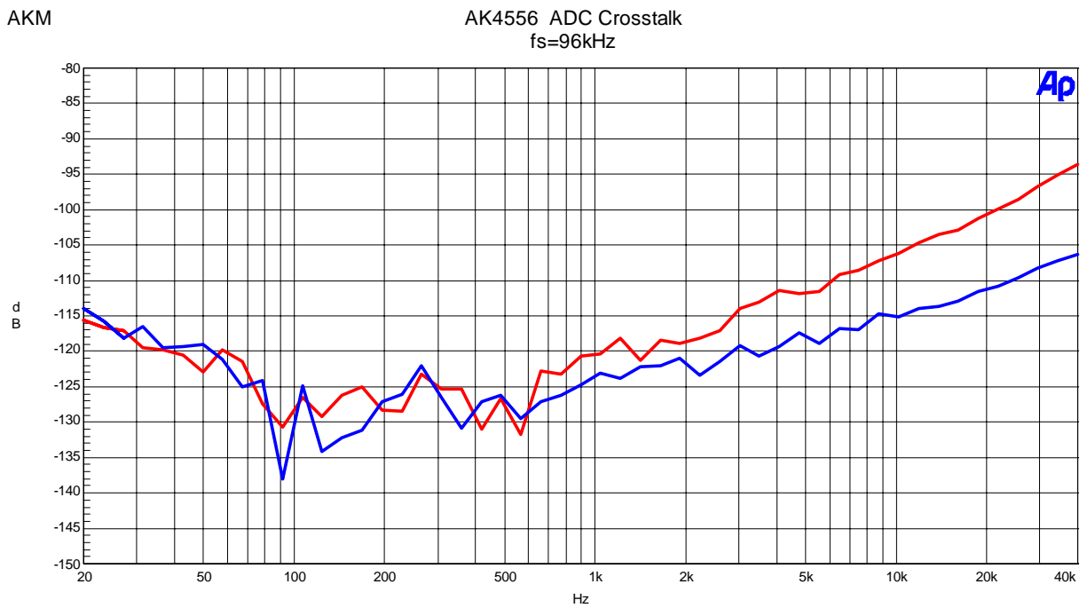
Figure 19. Crosstalk
