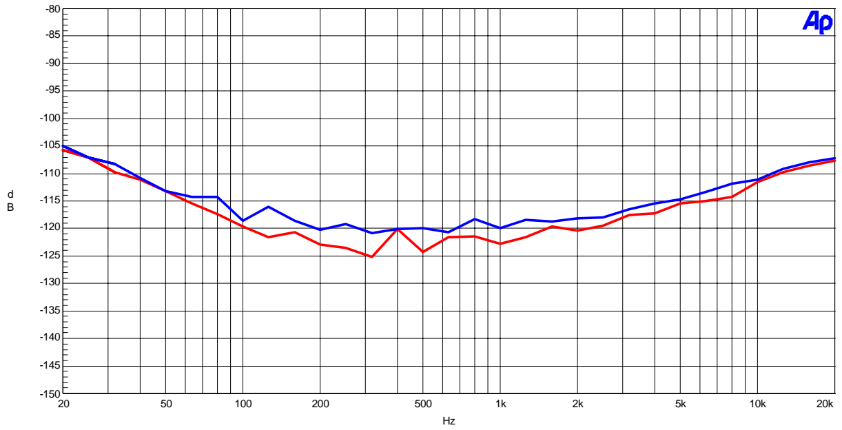
Figure 36. Crosstalk
