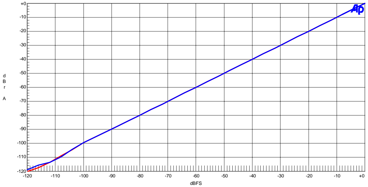
Figure 52. Linearity (fin=1kHz)
