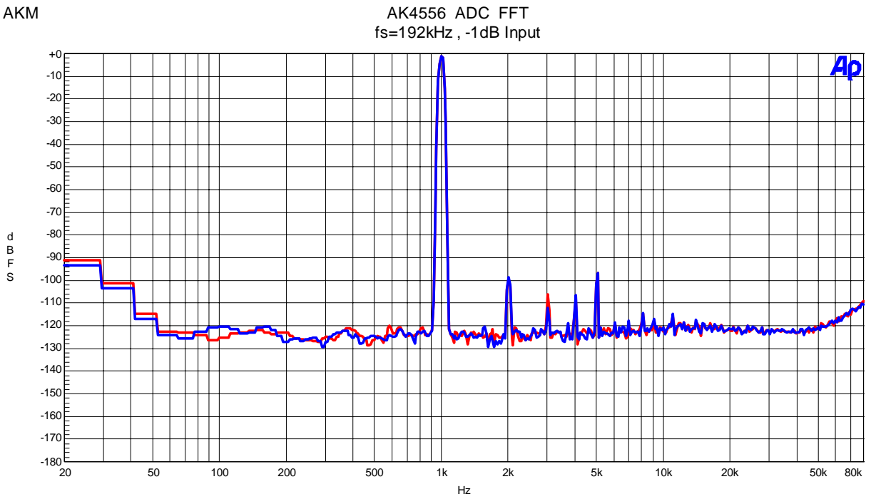
Figure 20. FFT (fin=1kHz , Input Level=-1dBFS)
