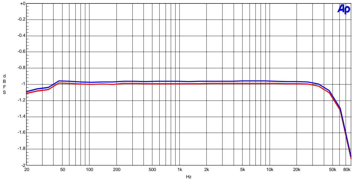
Figure 26. Frequency Response
