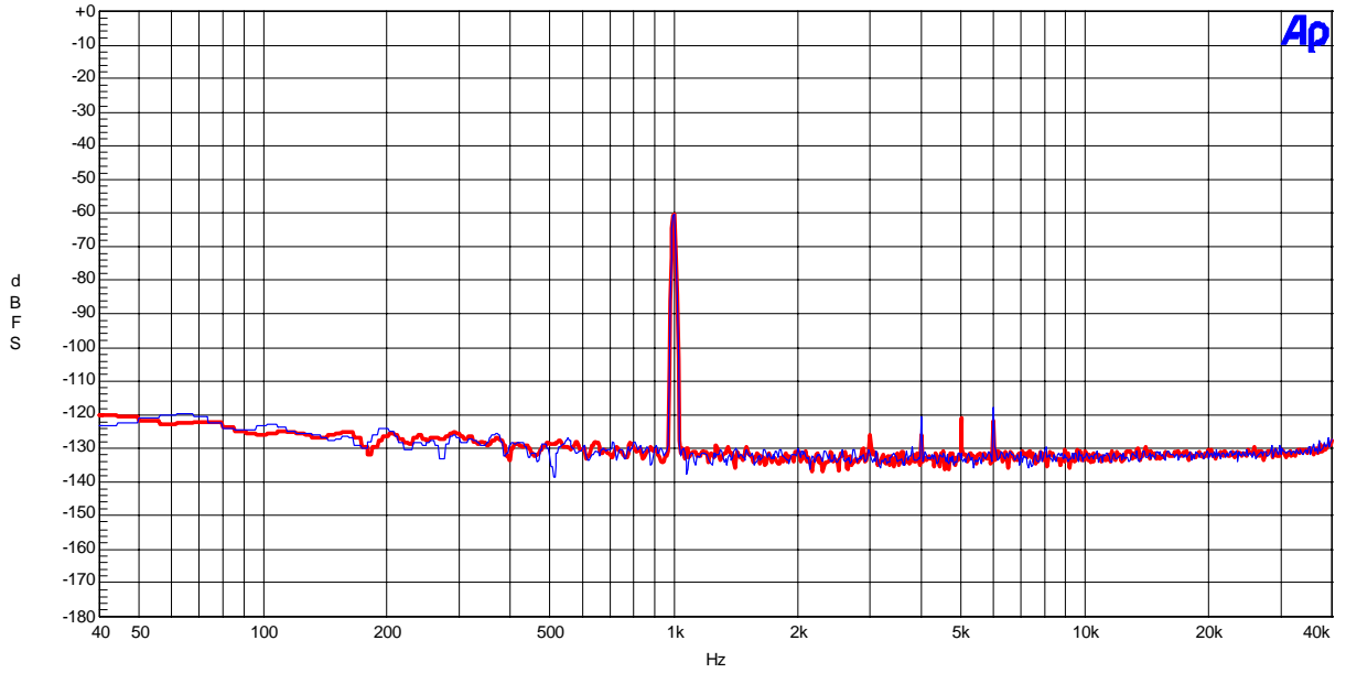
Figure 16 FFT (Input=-60dBFS, fin=1kHz)
