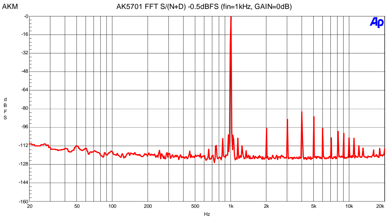
Figure 6. FFT Plot
