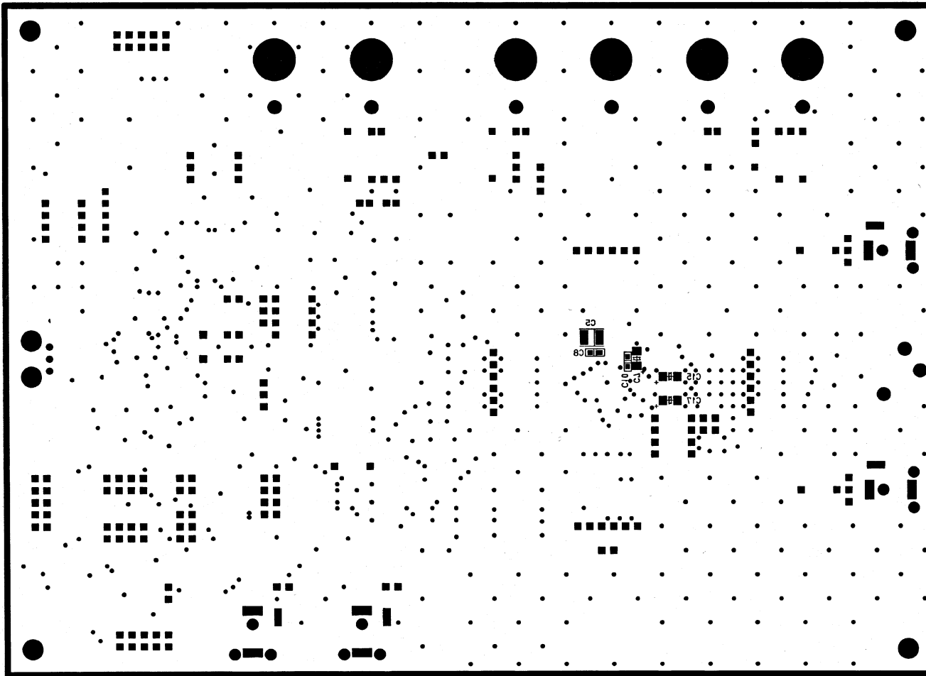
AKD2301-A-LS SILK
