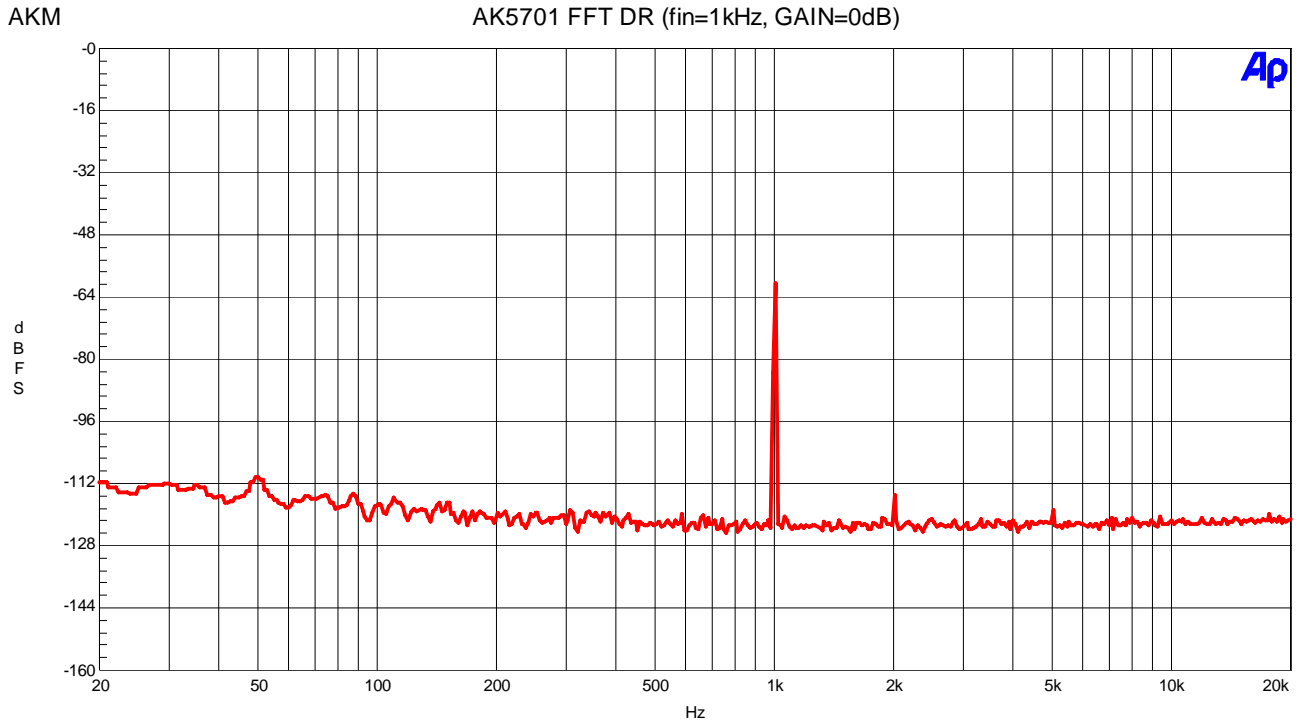
Figure 7. FFT Plot
