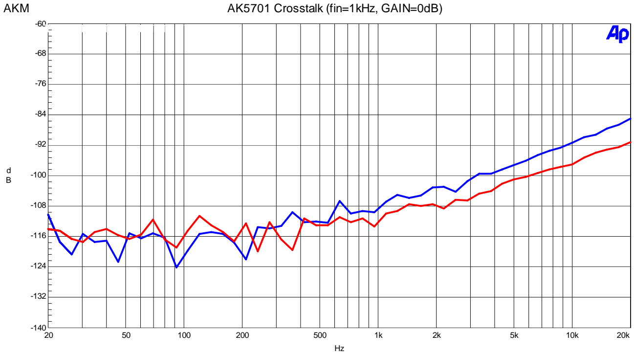
Figure 5. Crosstalk
