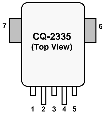
Figure 3. CQ-2335のピン配置
